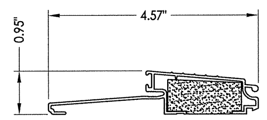
71 OUTSWING THRESHOLD Imperial
