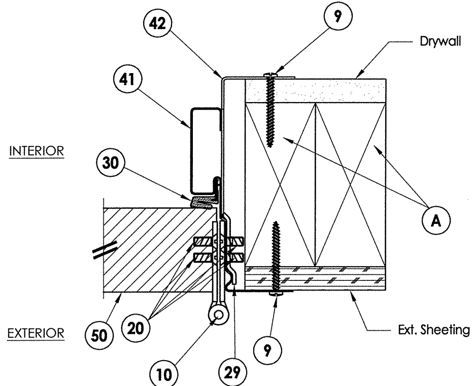
2 4 HORIZONTAL CROSS SECTION Optional 2X Stud Construction
