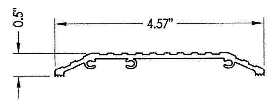
70 ADA THRESHOLD Imperial
