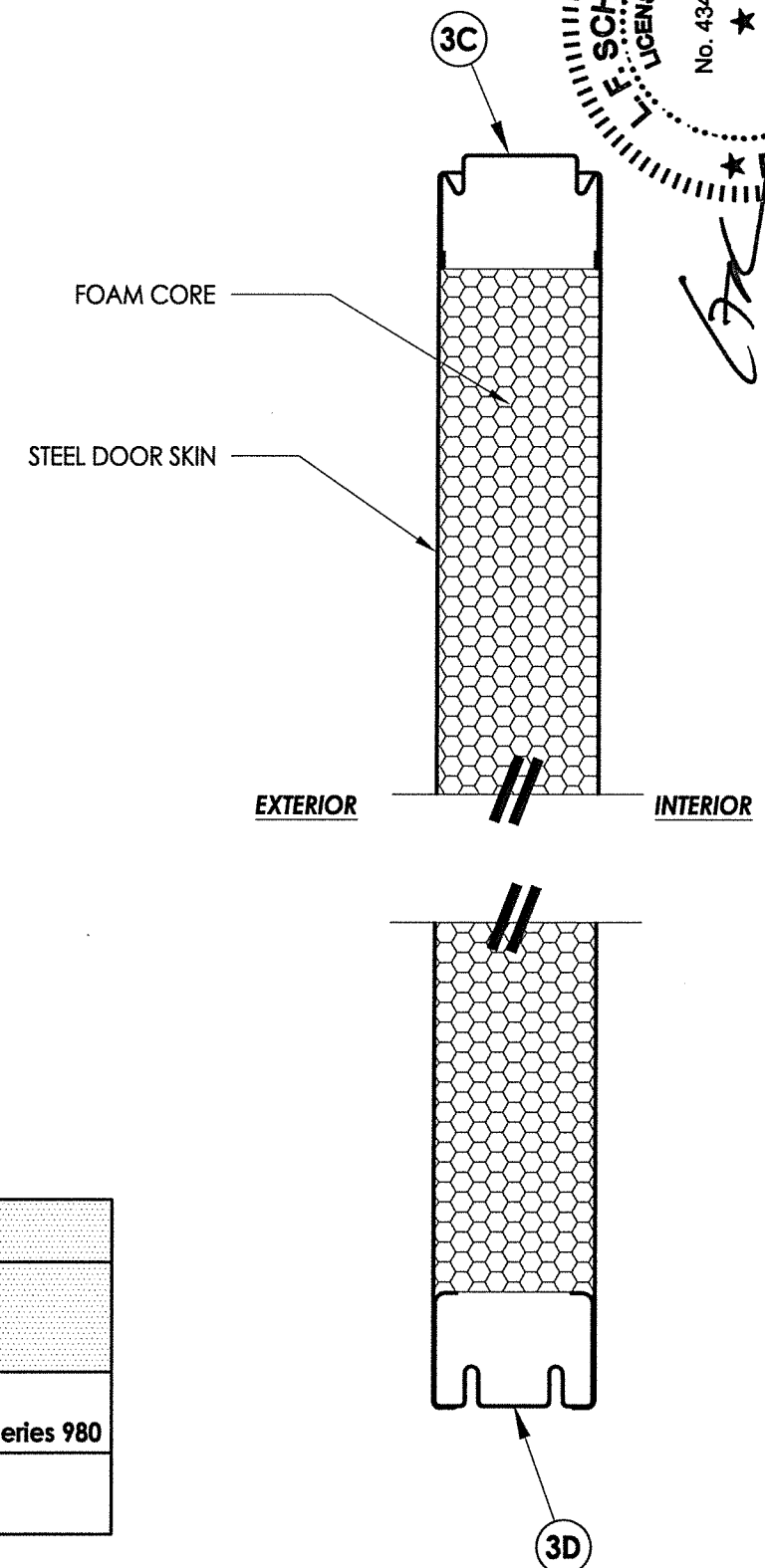
3D BOTTOM RAIL Steel edge door
