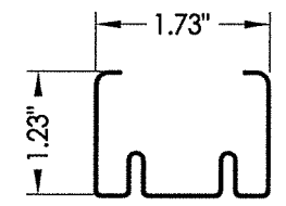
3D BOTTOM RAIL Steel edge door
