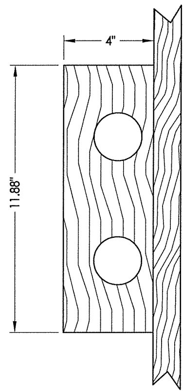
3B STILE Reinforcement
